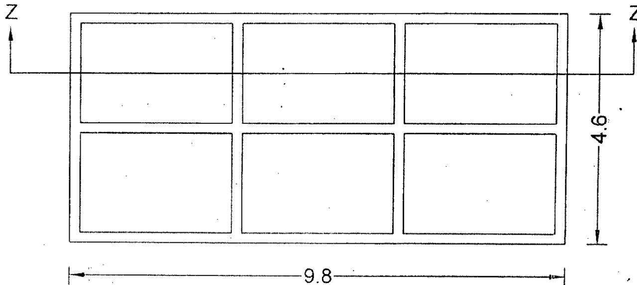
Dwg. A : Cattle Drinking Water Trough Plan
