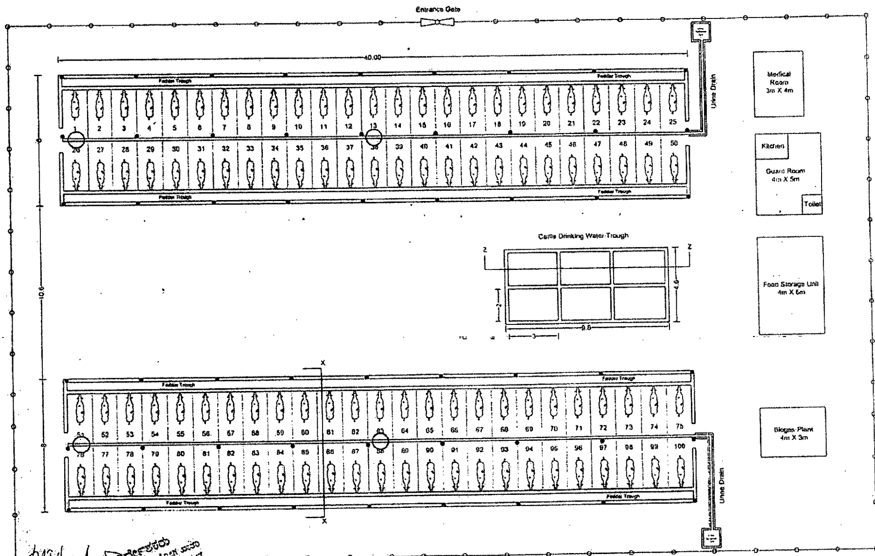
Dwg. : Plan of Cattle Shed 100 Cattle Capacity
