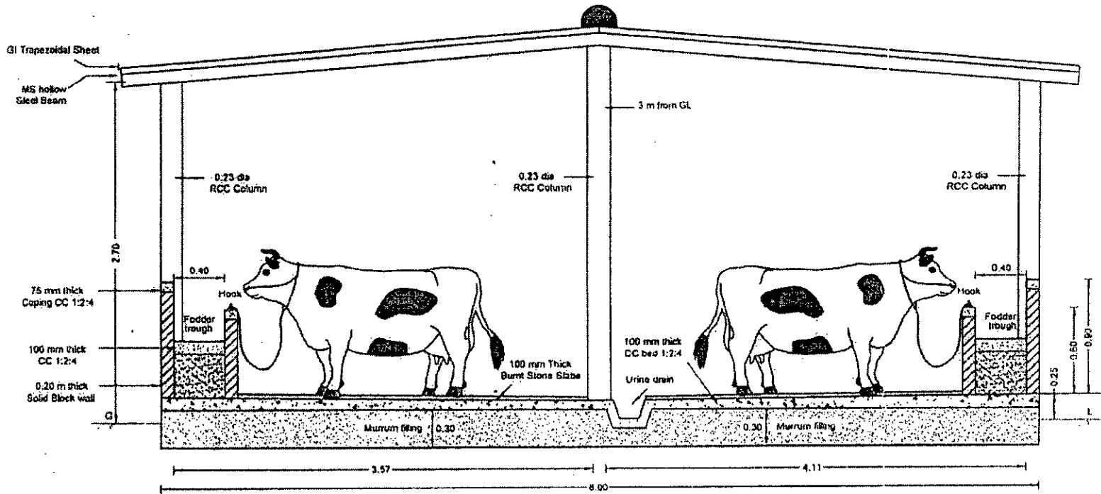
Fig a. Cross Section @ A-X
